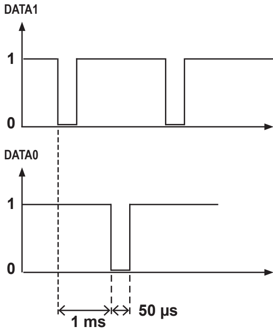
CHRONOGRAMMES - WIEGAND TIMES SERIES DIAGRAMM DES WIEGAND-PROTOKOLL-TIMINGS
